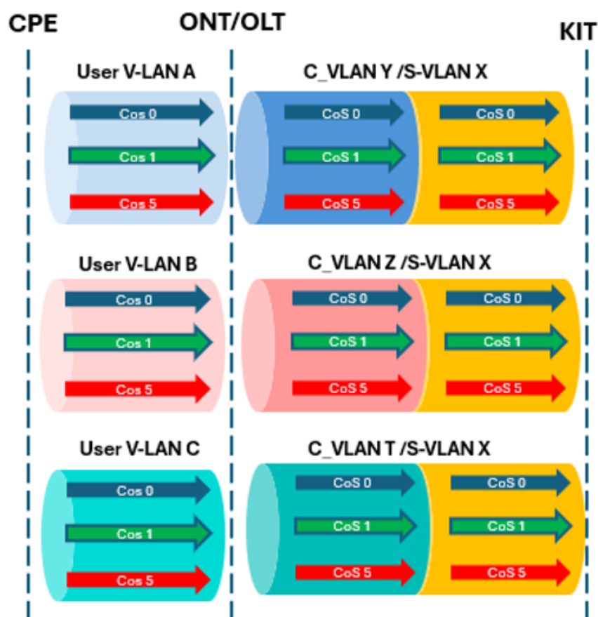
Figura 17 - Modello Multi-COS GBA/GBA IoT Multi C-VLAN
